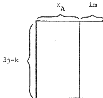
Fig. 8. The general form of A' . The left-hand r_A columns represent the column space of A (Fig. 4, on the right), and the right-hand im columns are the product-force vectors (Section 7) corresponding to the internal inextensional mechanisms. A' is square in the case ( rb = 0 ) of assemblies properly constrained to a rigid foundation.
