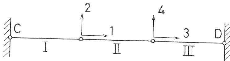
Fig. 6. An assembly of bars and joints in a plane.
